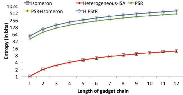
Figure 7. Entropy Comparison
